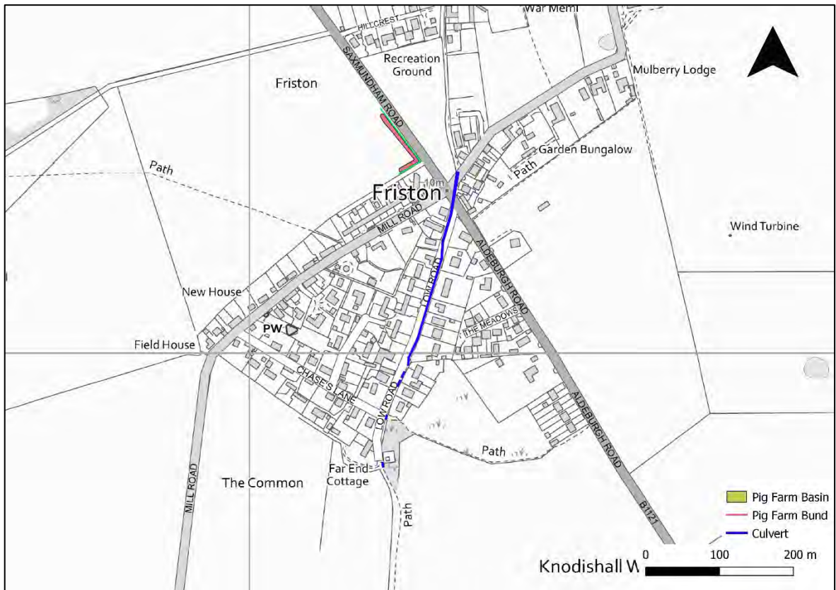
Figure 1-3 - Culvert and Flood Storage Area Location
