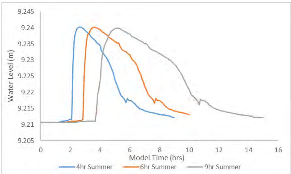
Figure 2-10 - Water Levels at Reporting Point at North of Low Road
