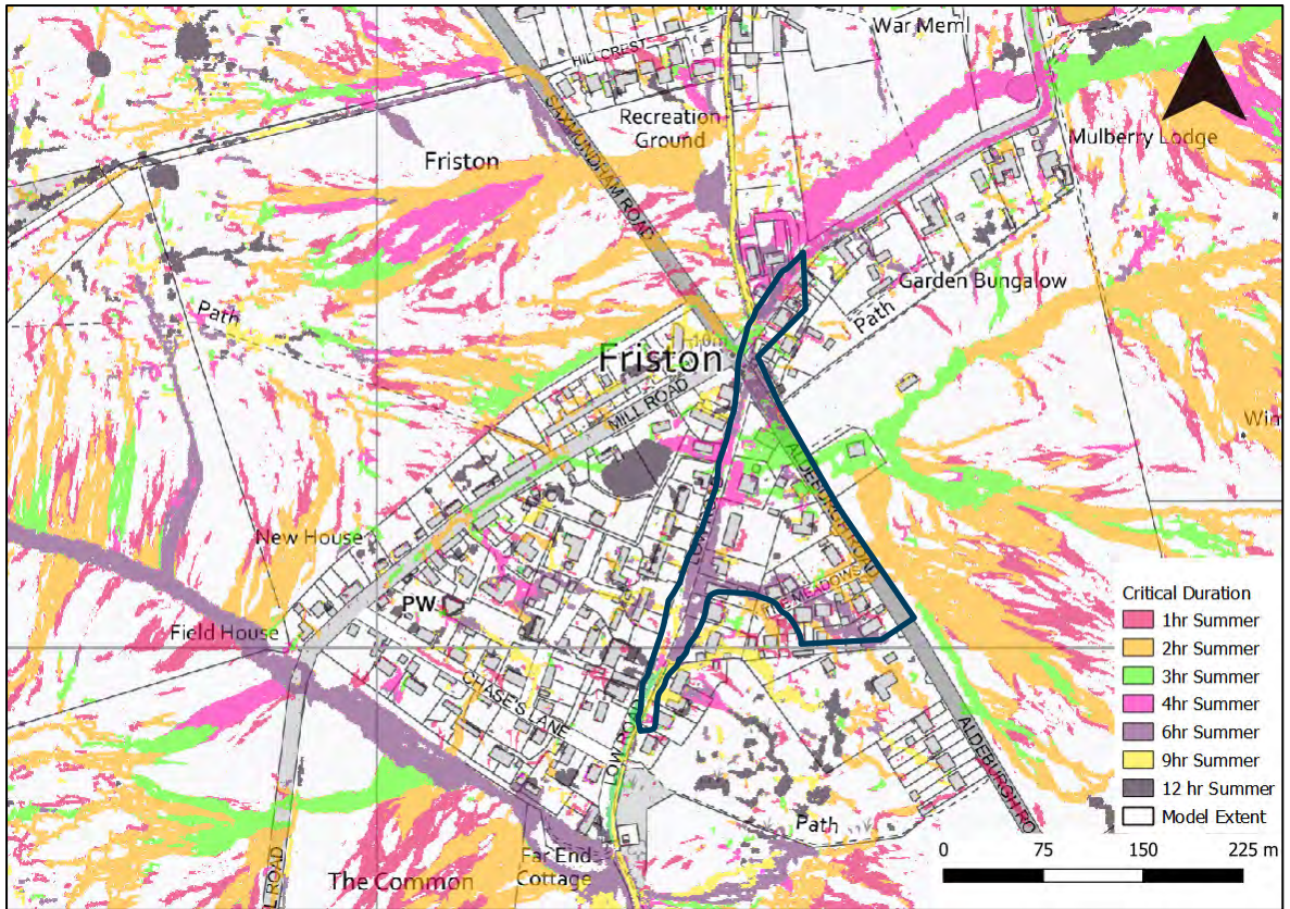
Figure 2-9 - Critical Duration for Summer events
