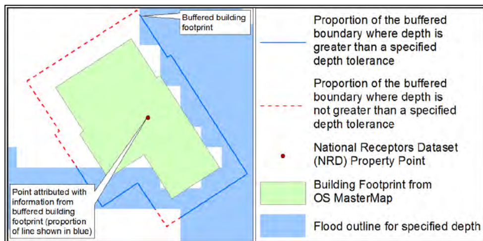
Figure 7-1 - Property Count Methodology (EA, July 2014)
