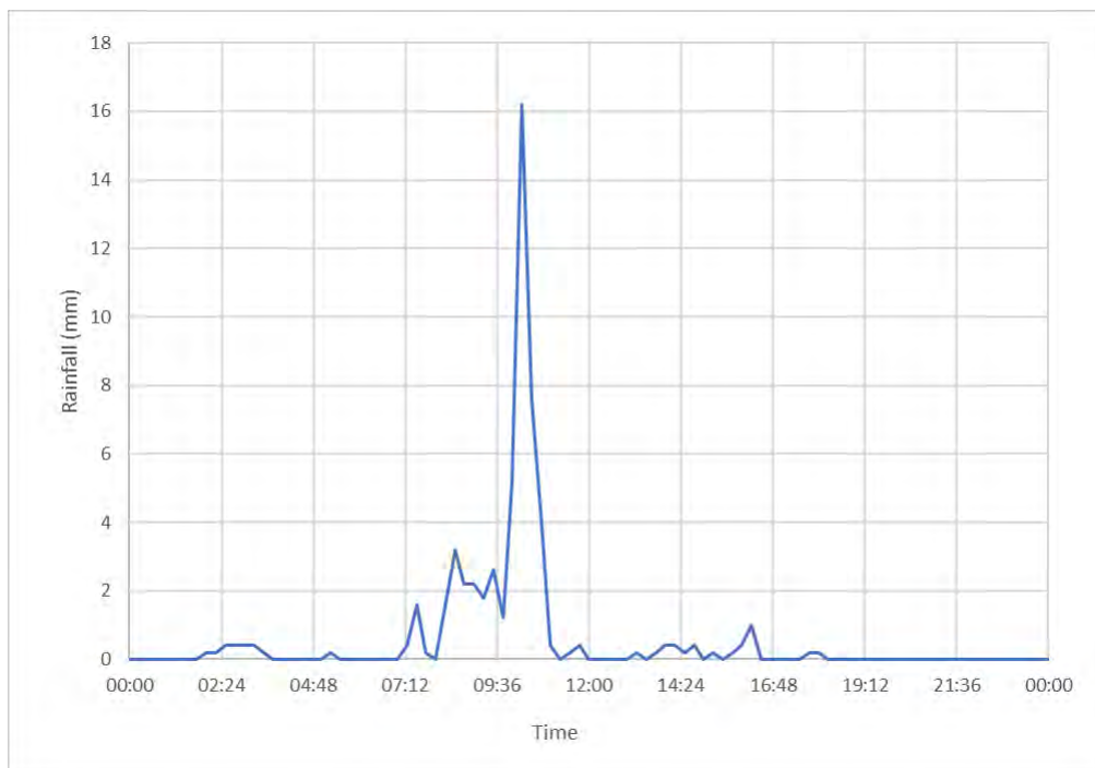
Figure 3-12 - Rainfall recorded on the 6 th of October 2019 at Thorpeness rainfall gauge
