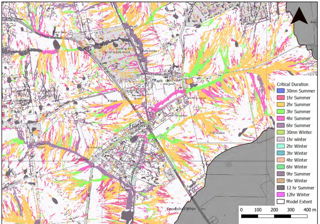
Figure 2-8 - Storm Duration Assessment for 1% AEP event
