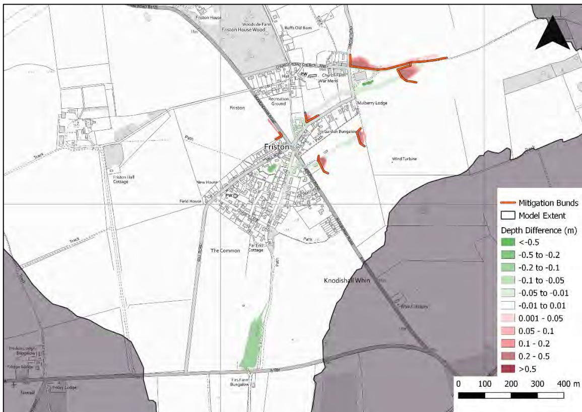
Figure 4-1 - Flood Prevention Measure 1, Depth Difference 1% AEP Event
