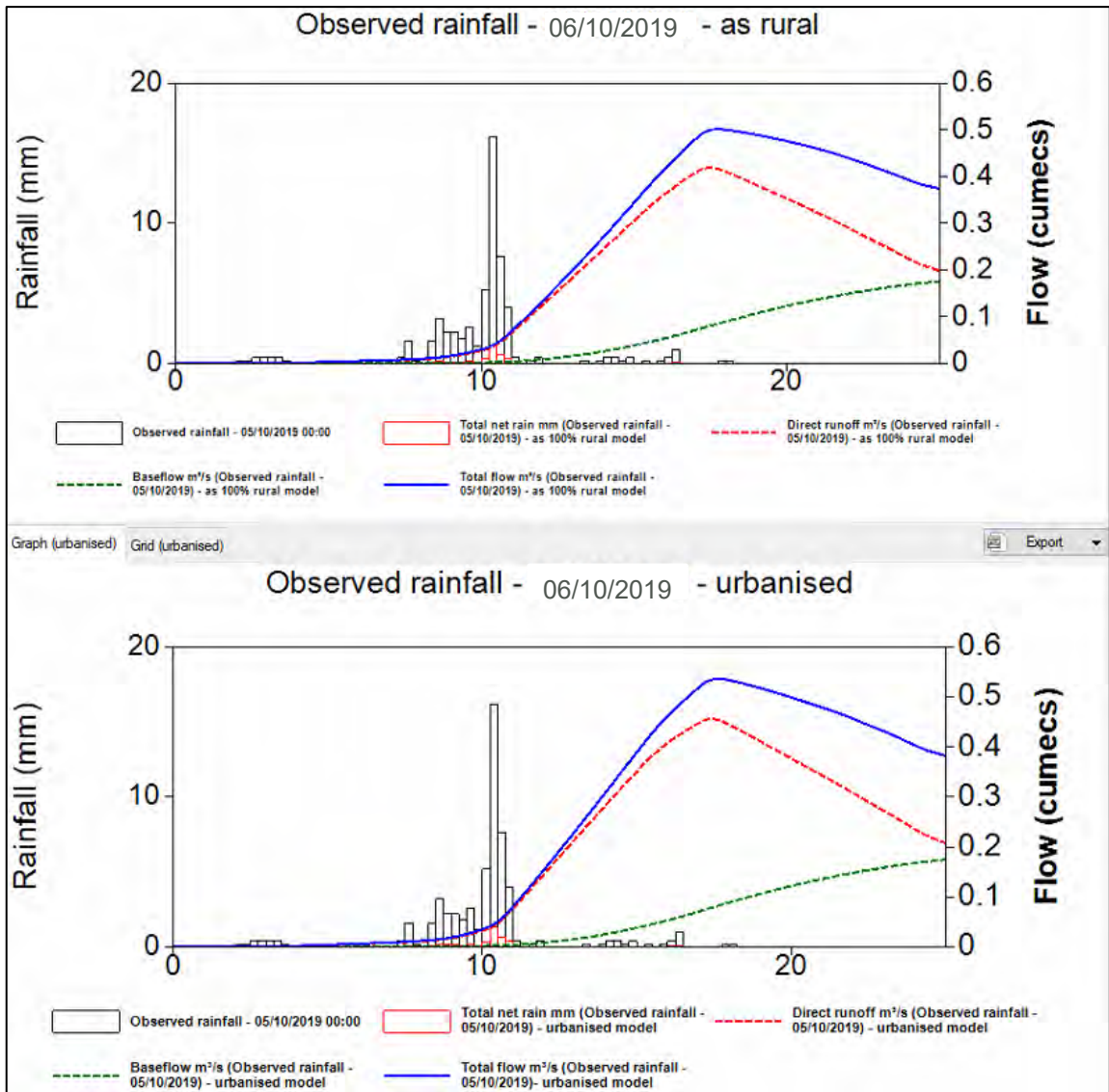
Figure 2-5 - ReFH2.3 Observed Event Rainfall and Runoff
