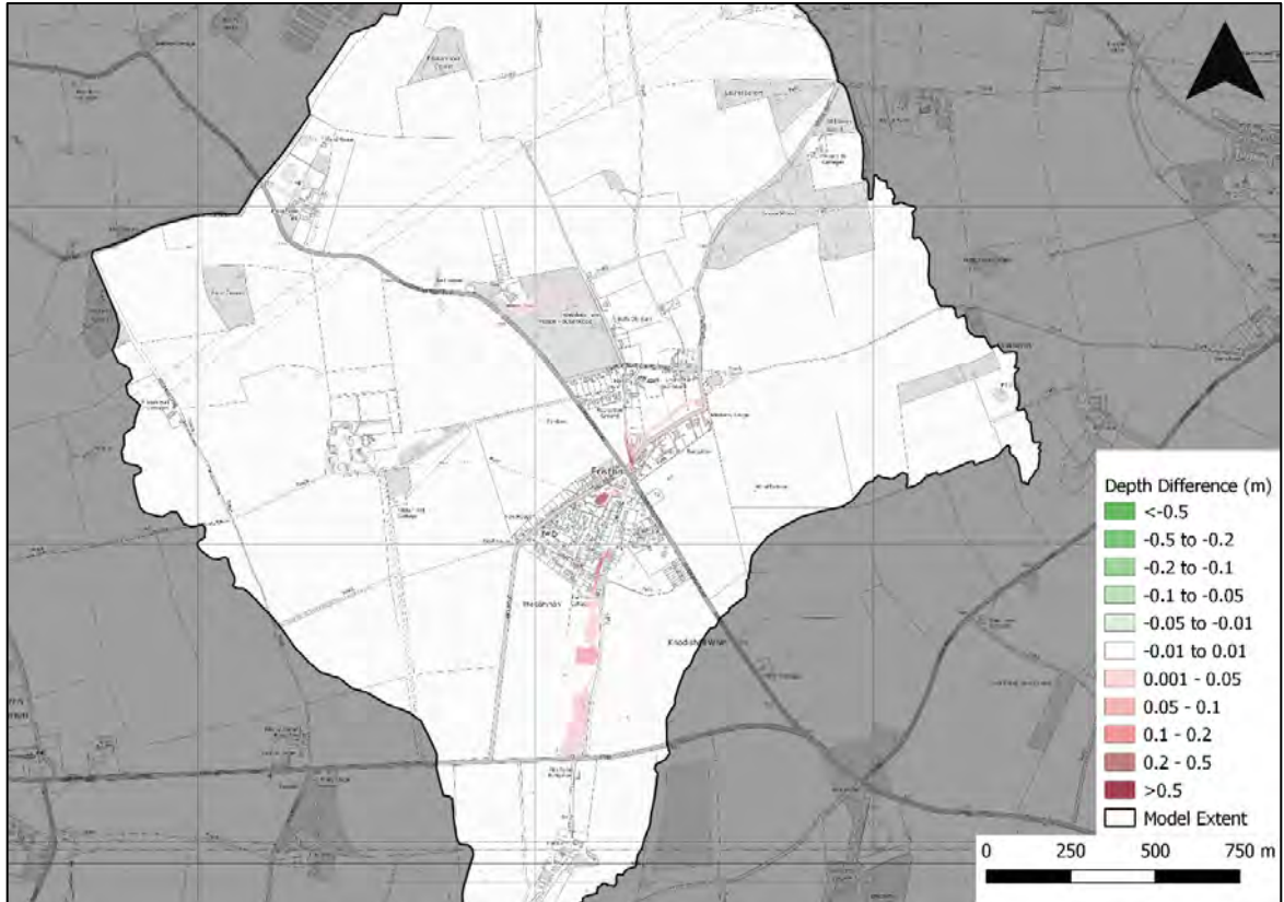
Figure 6-2 - Baseline Scenario Vs Do-Nothing, 1% AEP Rainfall Event.
