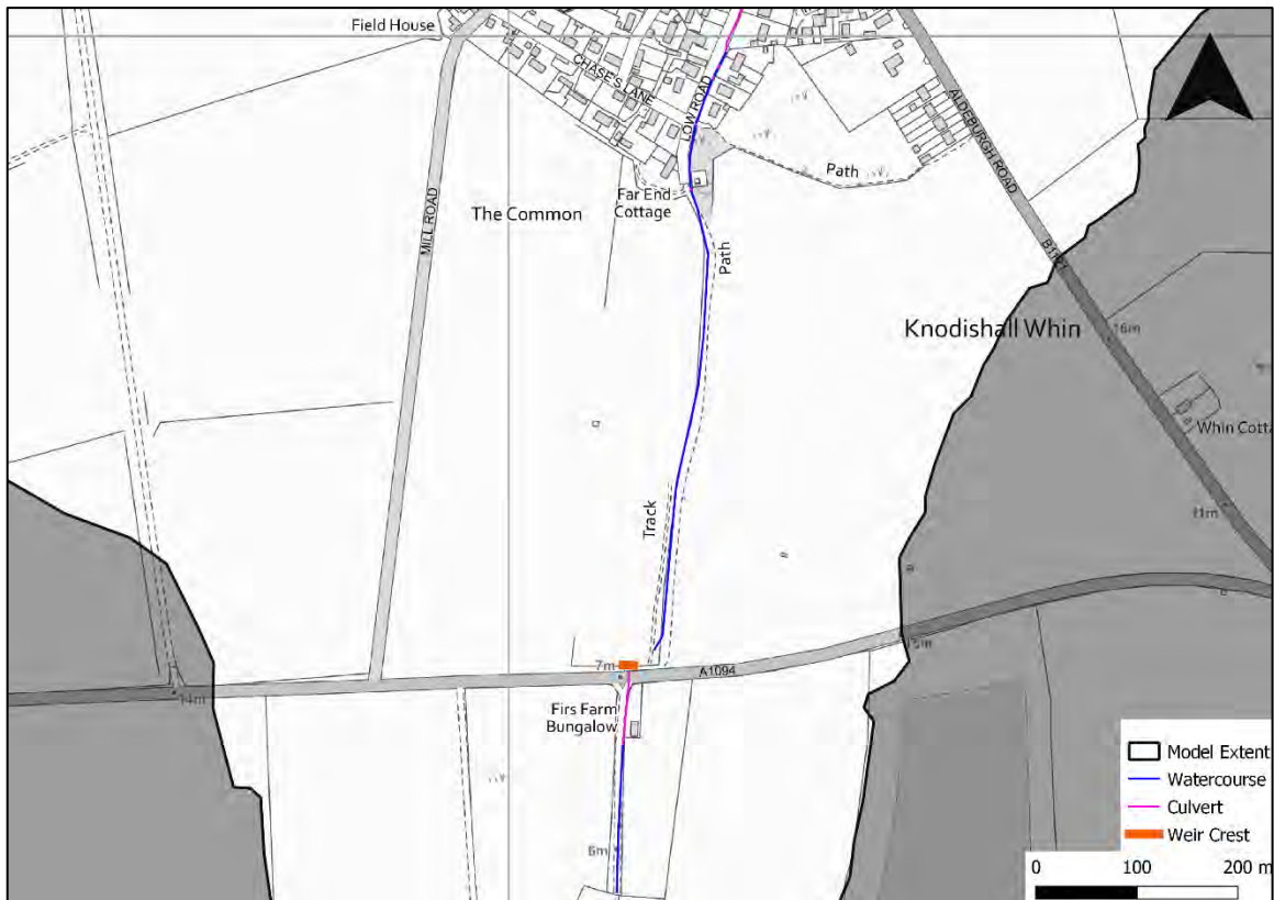
Figure 2-3 - A1094 Weir Location
