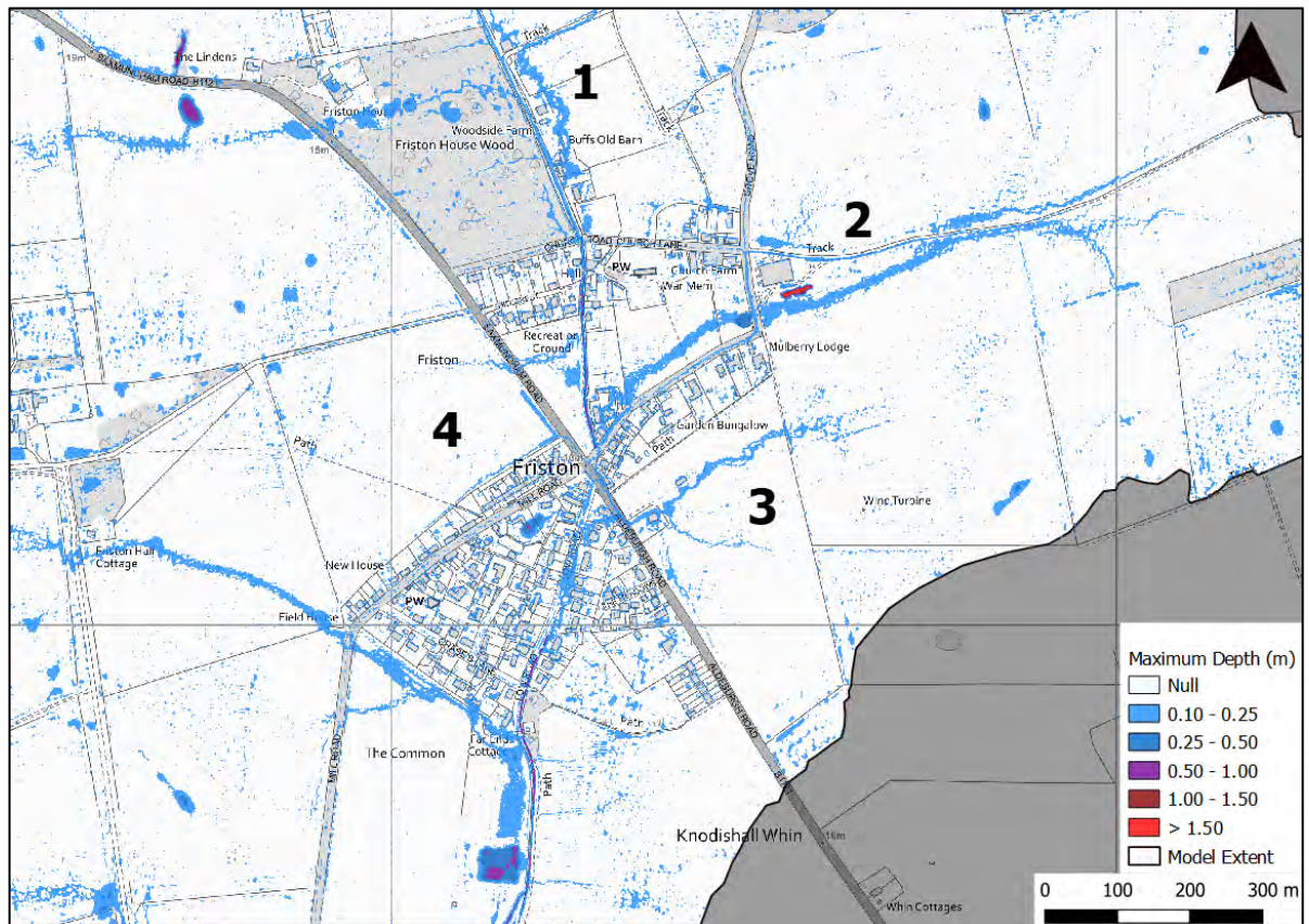
Figure 3-1 - Key Flow Paths in Friston (Baseline 1% AEP Rainfall Event)
