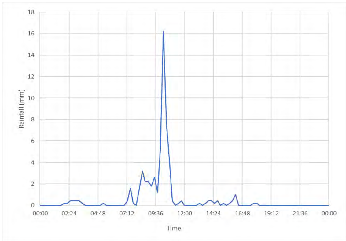
Figure 2-4 - Rainfall recorded on the 6 th of October 2019 at Thorpeness rainfall gauge
