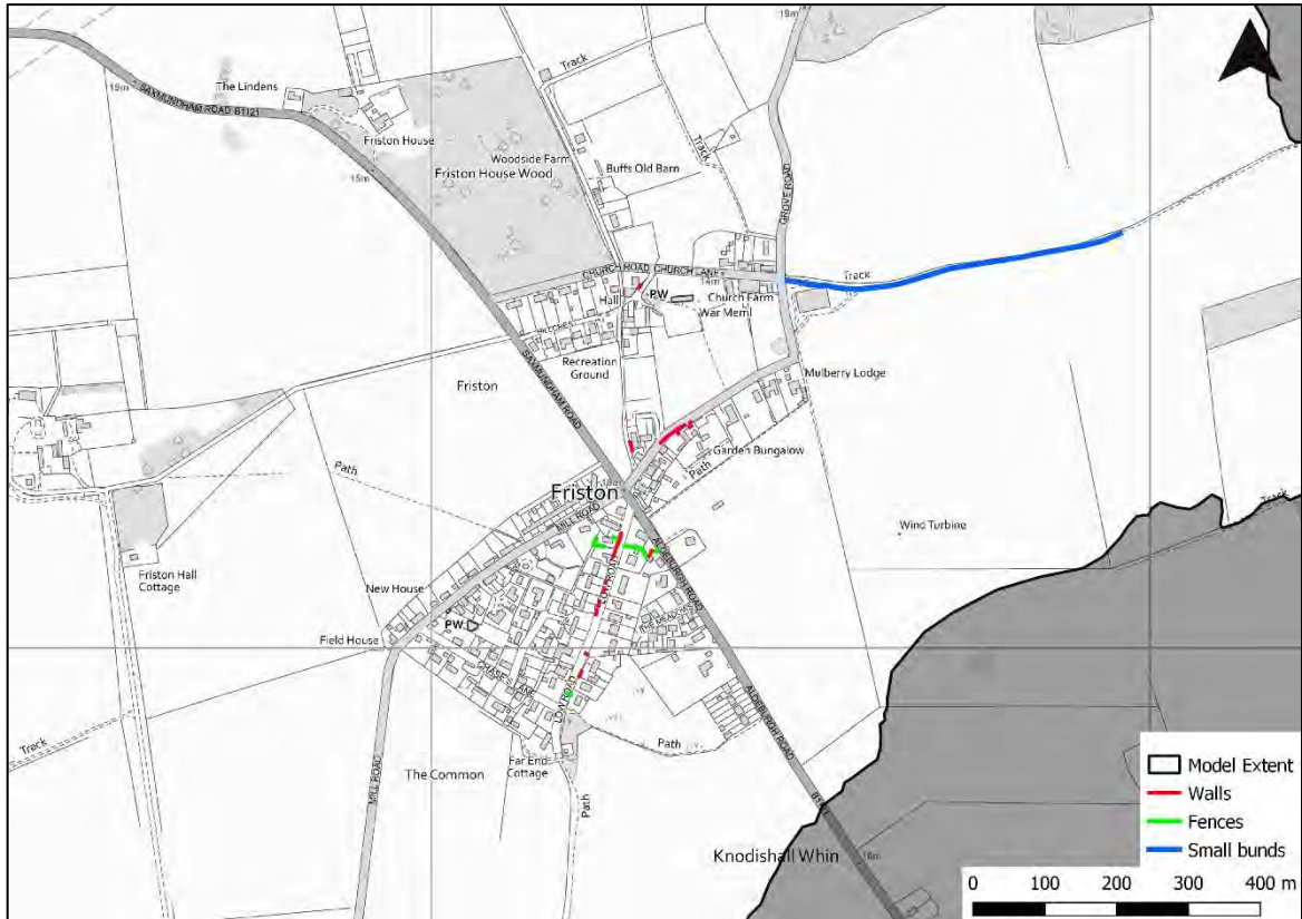
Figure 3-4 - Locations of walls and fences
