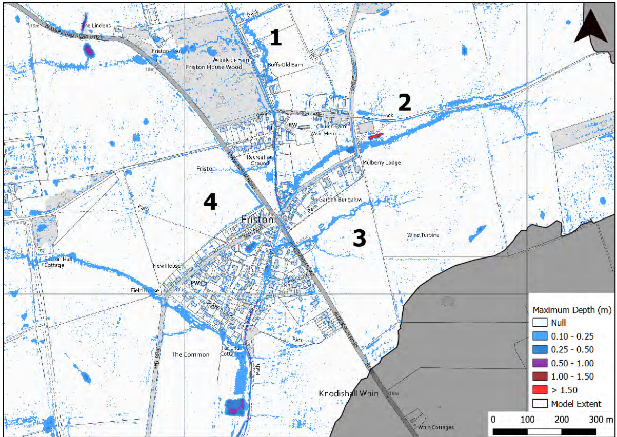
Figure 4-1 - Key Flow Paths in Friston (1% AEP Rainfall Event)
