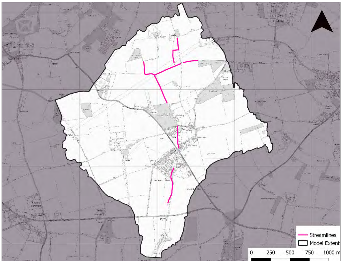
Figure 2-6 – Representation of Baseflow
